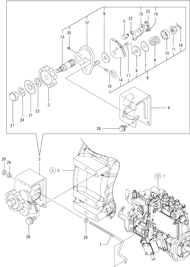
Fig.16. ENGINE CONTROL DEVICE
