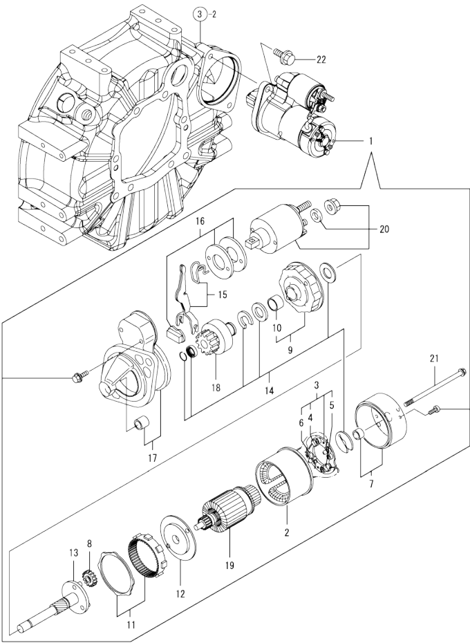
Fig.17. STARTING MOTOR
