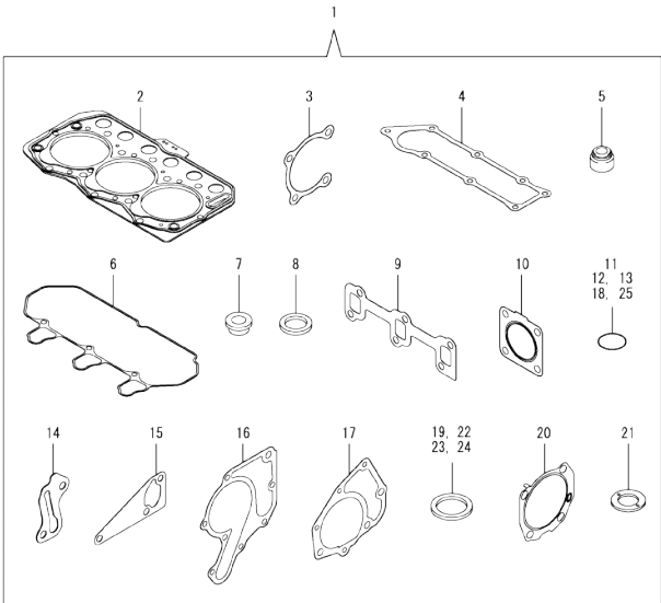
Fig.20. GASKET SET
